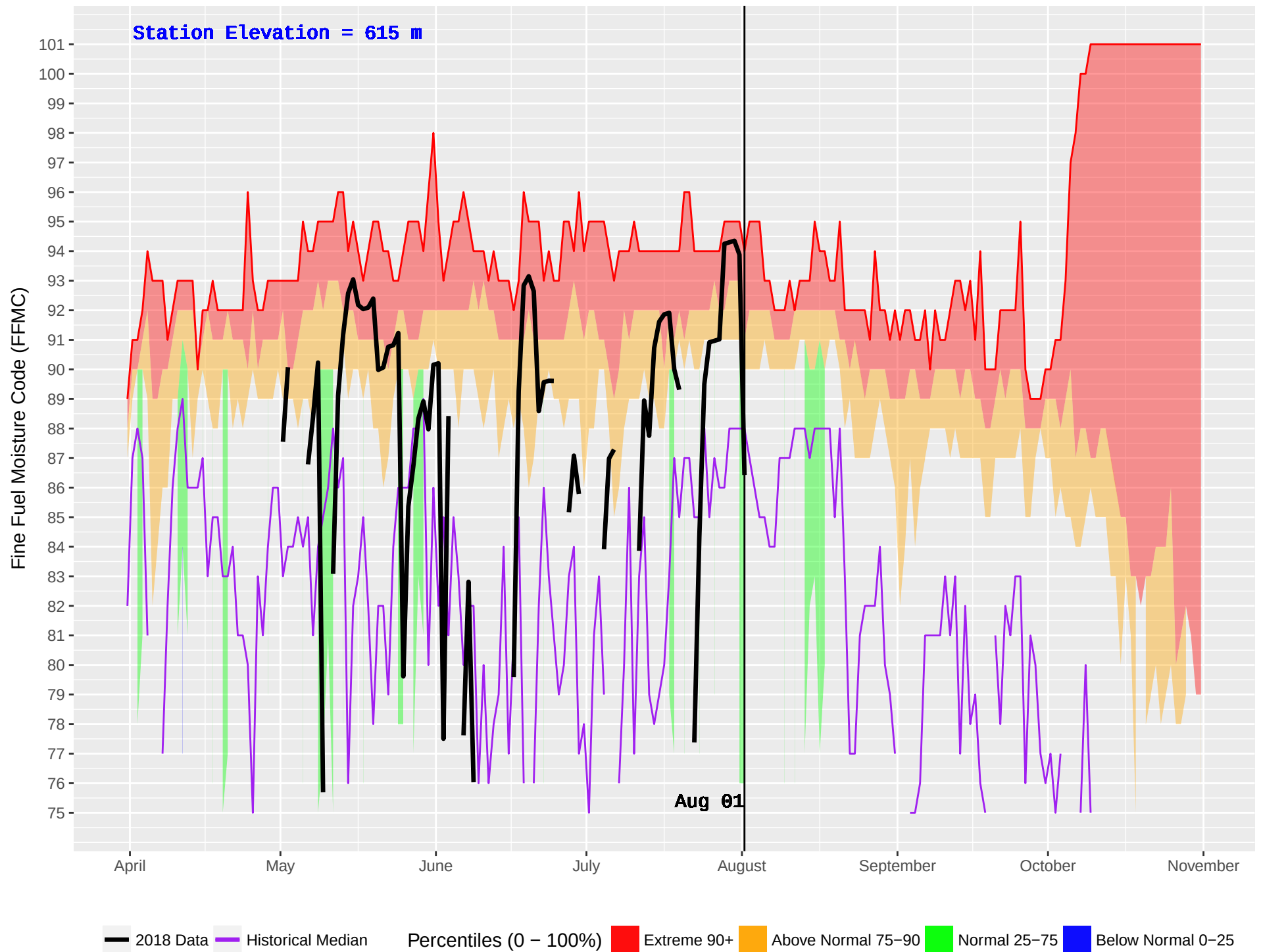
HIXON (187) : Historical (1976–2016) and Current (2018) Daily Fine Fuel Moisture Code (FFMC)
