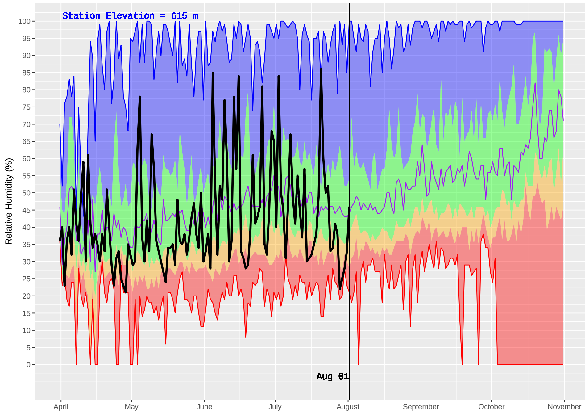
HIXON (187) : Historical (1976–2016) and Current (2018) Daily Relative Humidity
