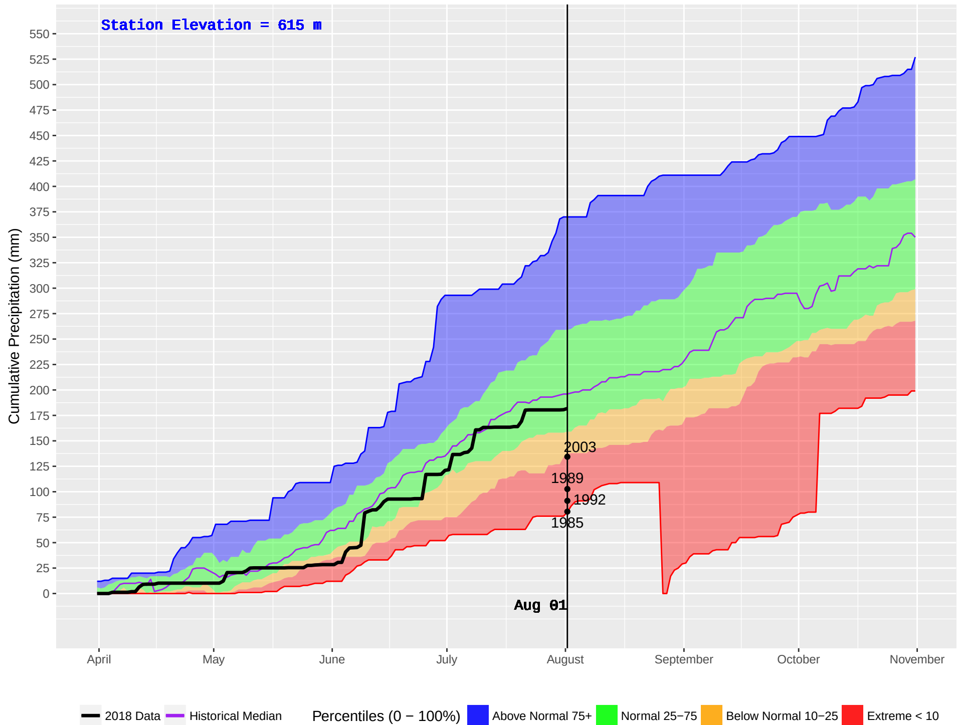
HIXON (187) : Historical (1976–2016) and Current (2018) Daily Cumulative Precipitation
