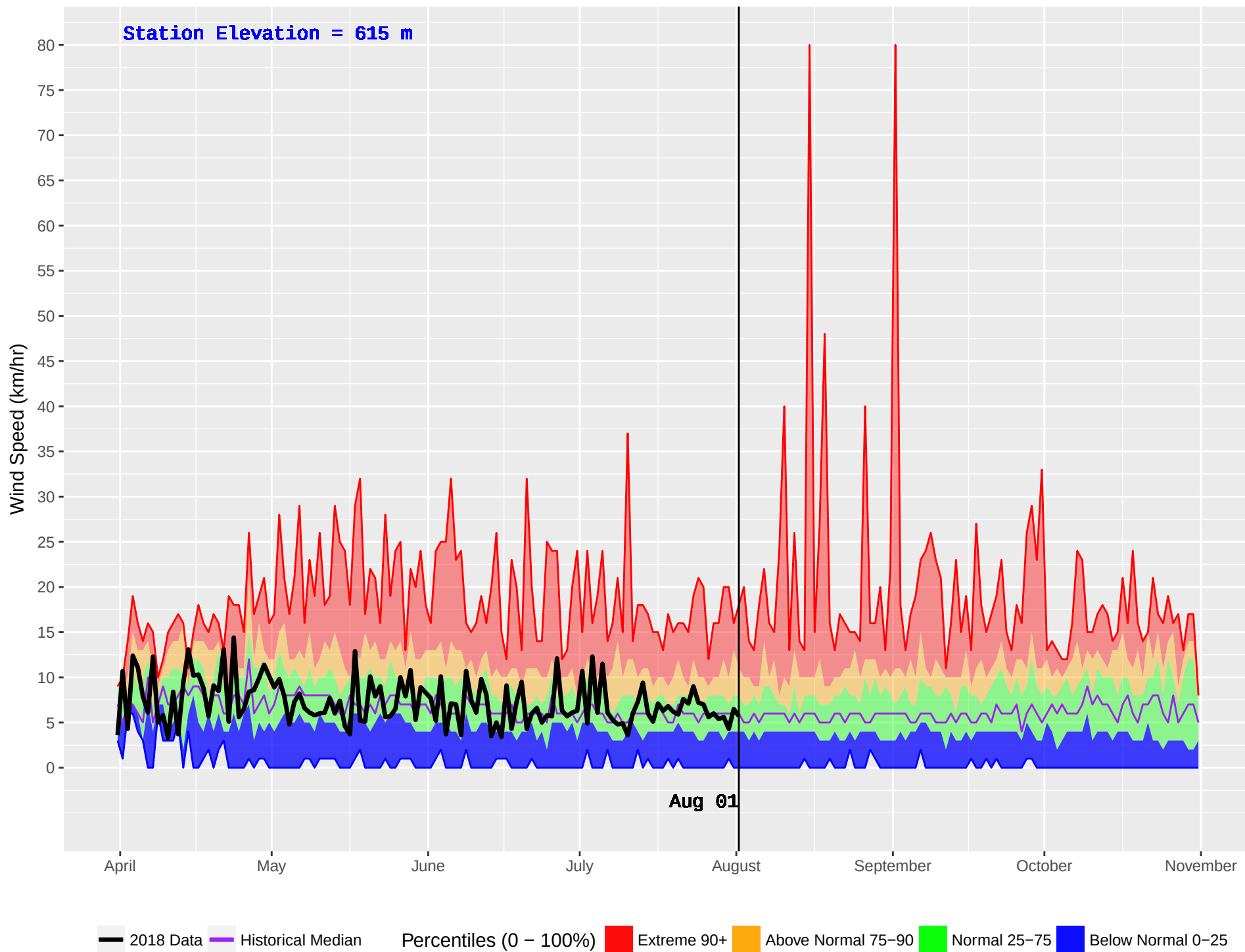
HIXON (187) : Historical (1976–2016) and Current (2018) Daily Wind Speed
