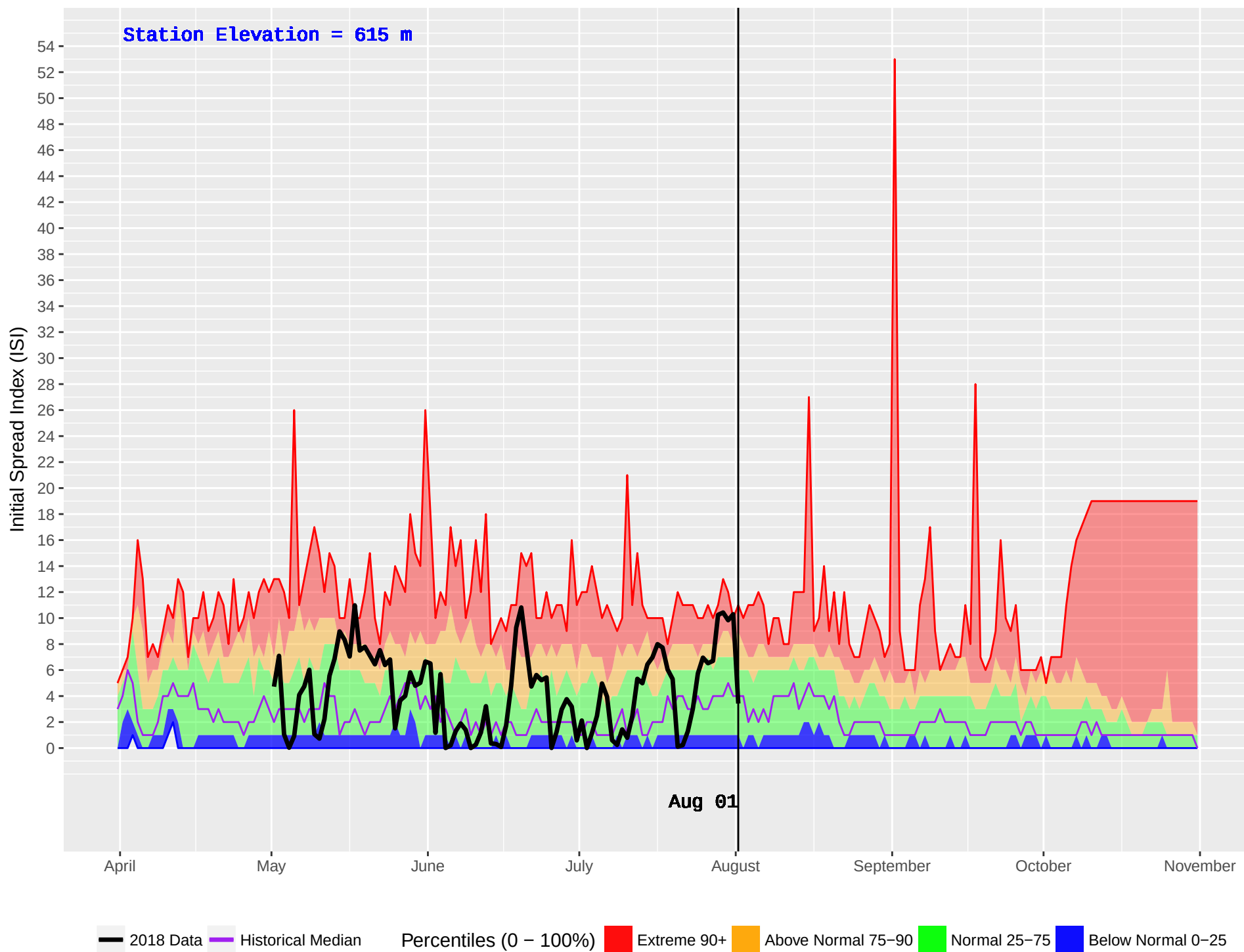
HIXON (187) : Historical (1976–2016) and Current (2018) Daily Initial Spread Index (ISI)
