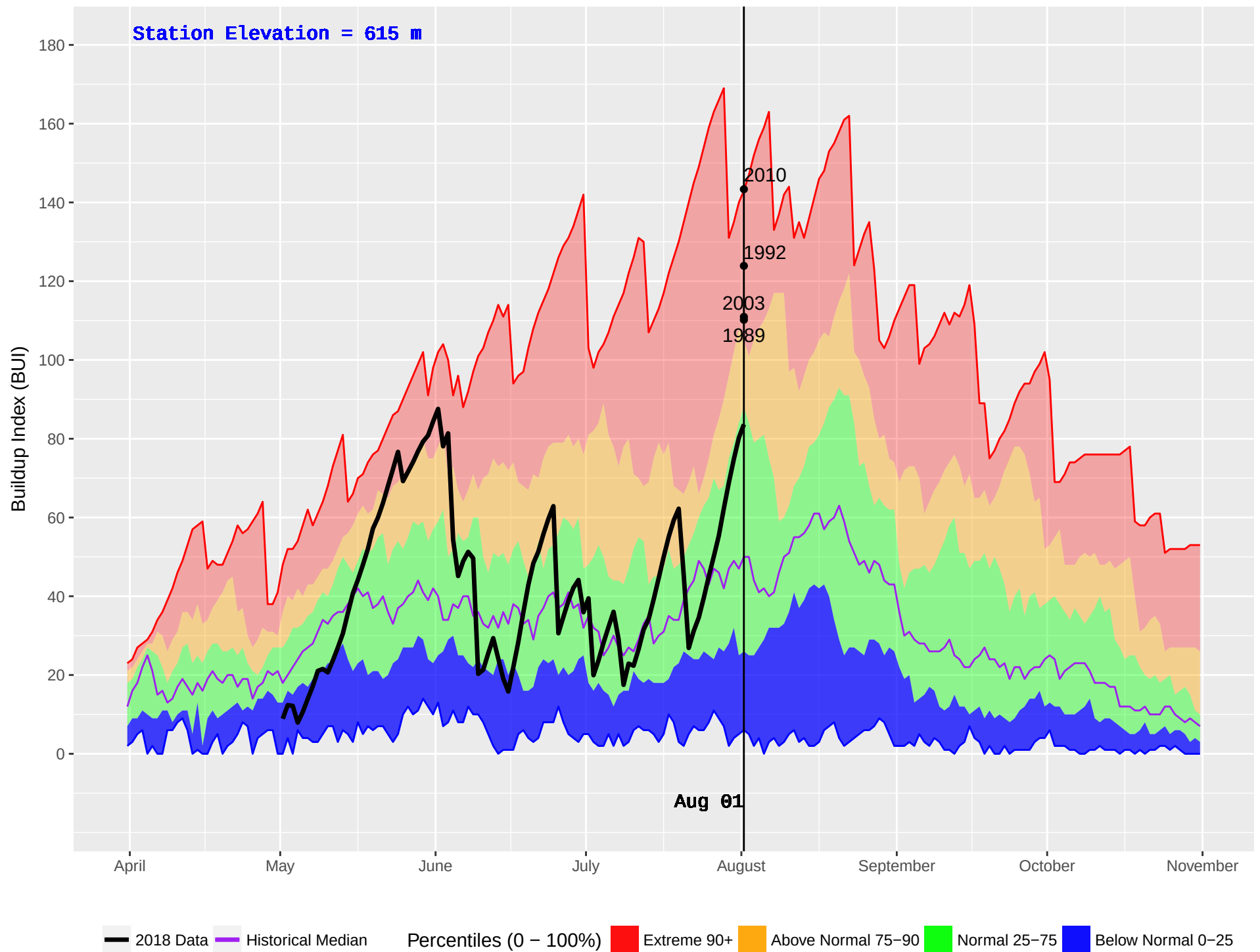
HIXON (187) : Historical (1976–2016) and Current (2018) Daily Buildup Index (BUI)
