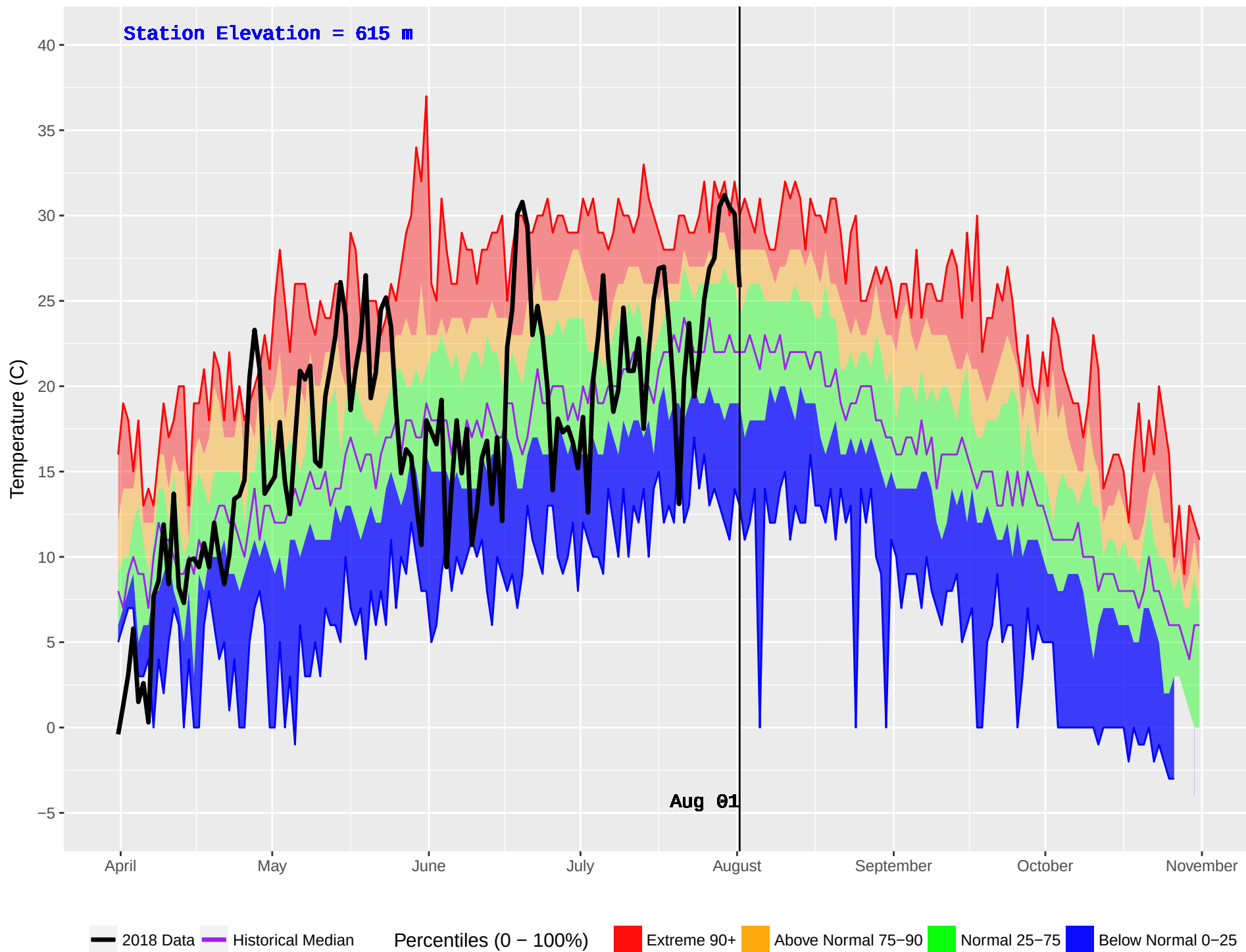
HIXON (187) : Historical (1976–2016) and Current (2018) Daily Temperature
