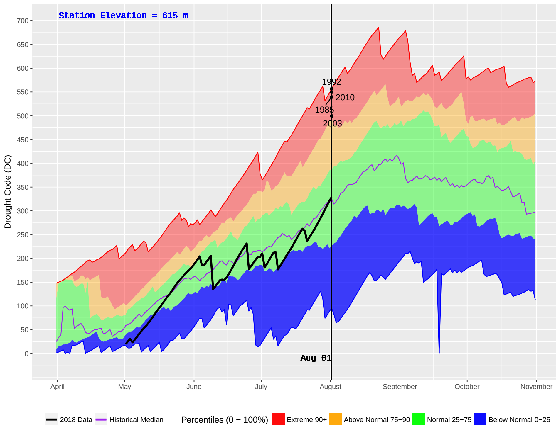
HIXON (187) : Historical (1976–2016) and Current (2018) Daily Drought Code (DC)
