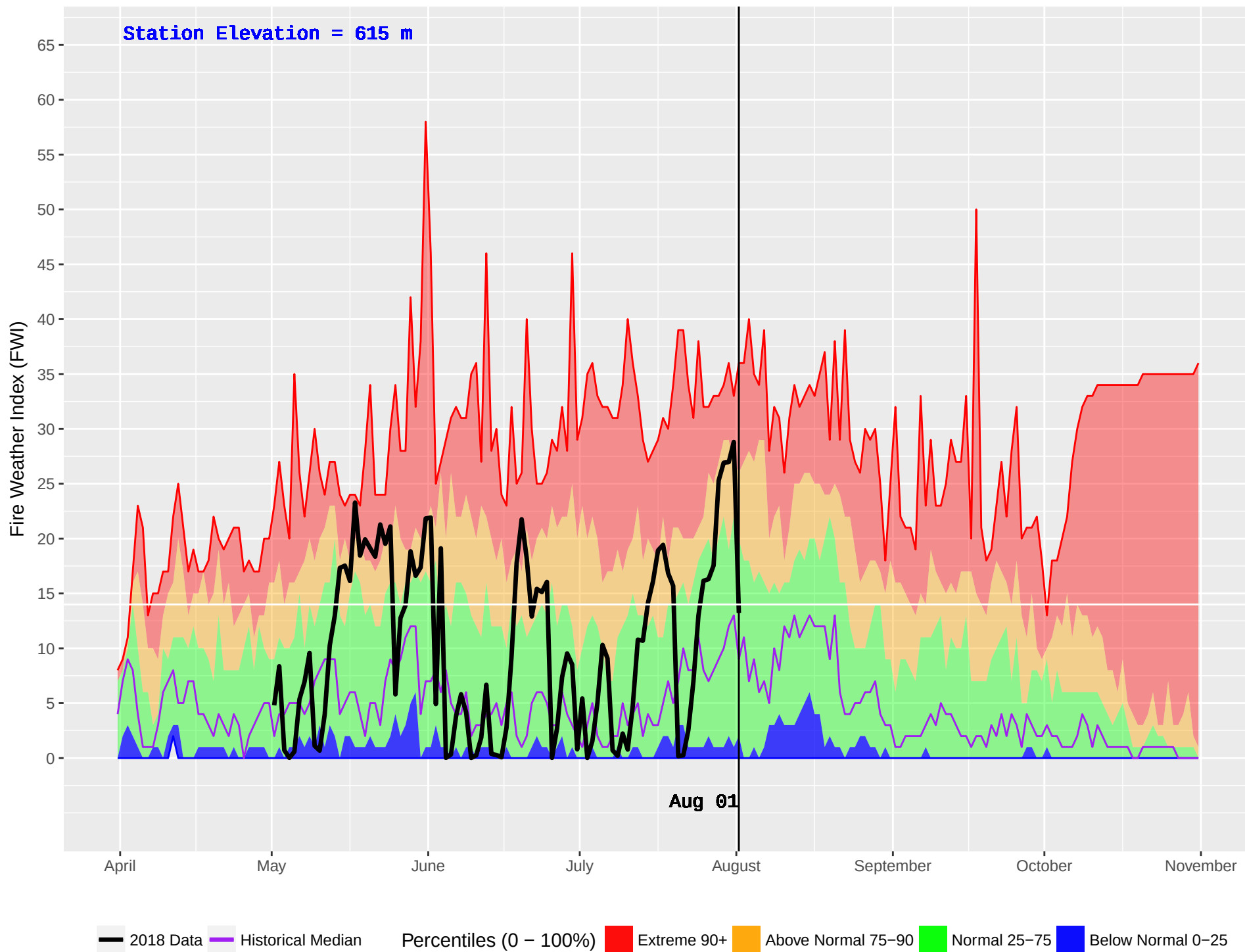
HIXON (187) : Historical (1976–2016) and Current (2018) Daily Fire Weather Index (FWI)
